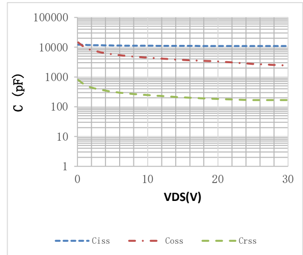
Fig.2 Capacitance Characteristics
